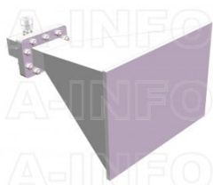
LB-229-15-C-7SPO Standard Gain Horn Antenna 3.3-4.9GHz 15dB Gain 7mm
