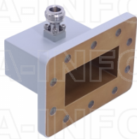
229WCAN Right Angle Rectangular Waveguide to Coaxial Adapter 3.3-4.9GHz WR229 to N Type Female
