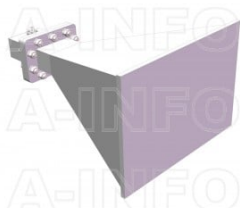
LB-229-15-C-SFSPO Standard Gain Horn Antenna 3.3-4.9GHz 15dB Gain SMA Female
